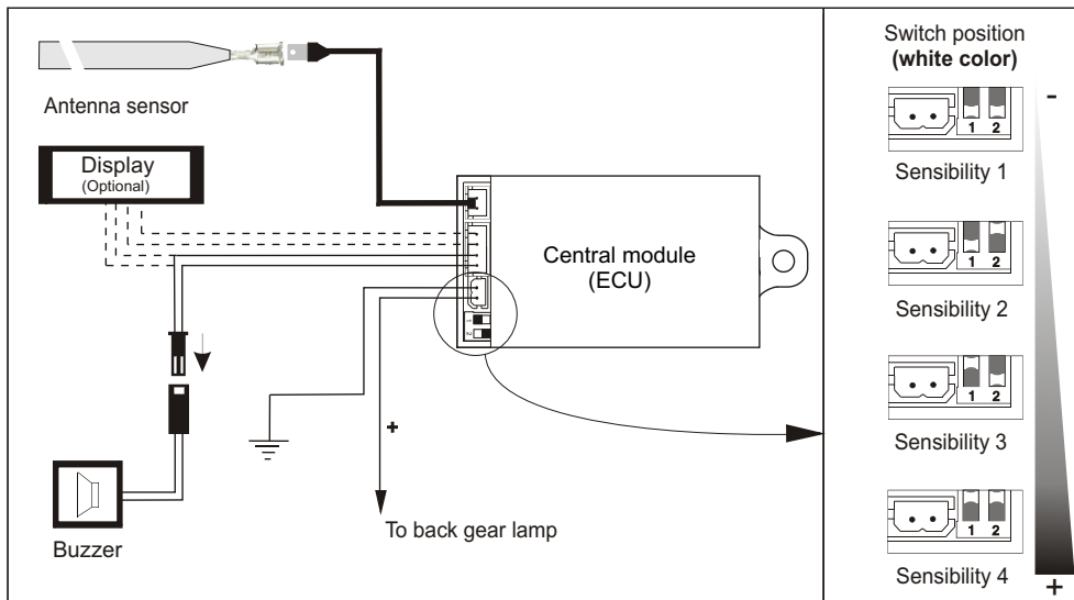
Blocks schematic
